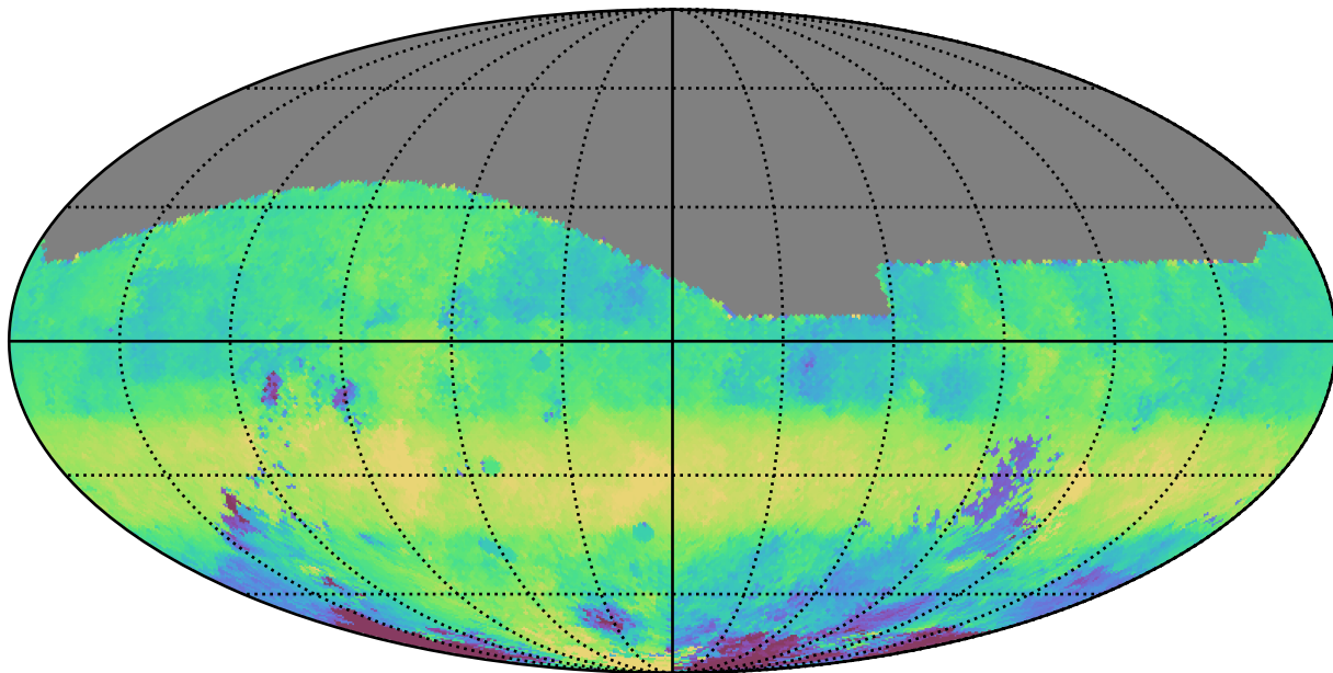
too_elab_r16_d2_gz_v3.4_10yrs All sky g band: Median HA
