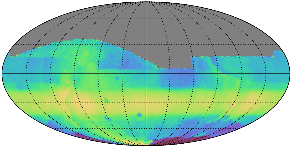
too_elab_r16_d2_gz_v3.4_10yrs All sky all bands: Median HA
