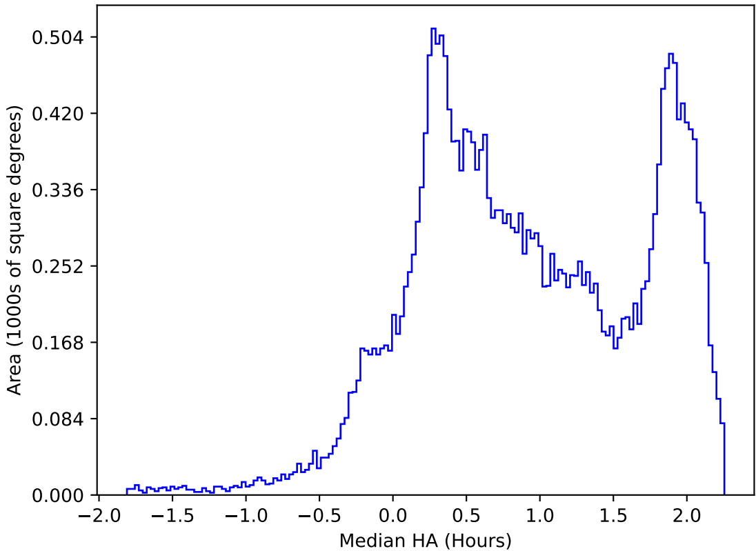
too_elab_r16_d2_gz_v3.4_10yrs All sky all bands: Median HA
