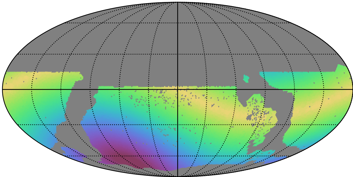
too_elab_r16_d2_gz_v3.4_10yrs WFD y band: Max solarElong
