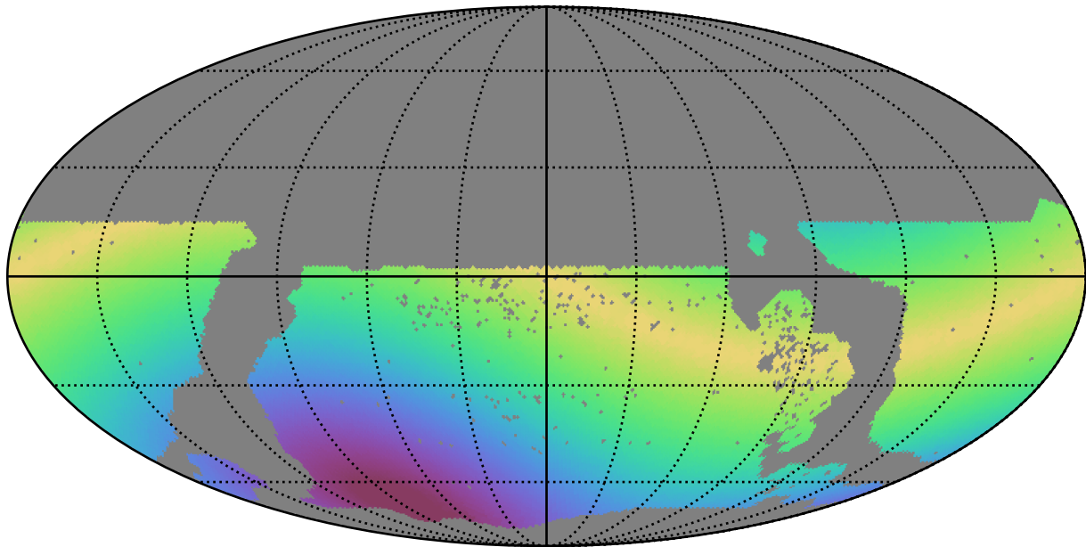
too_elab_r16_d2_gz_v3.4_10yrs WFD r band: Max solarElong
