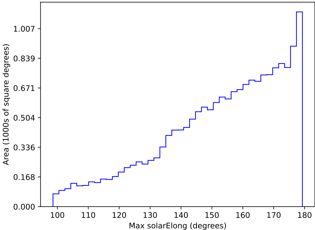
too_elab_r16_d2_gz_v3.4_10yrs WFD r band: Max solarElong
