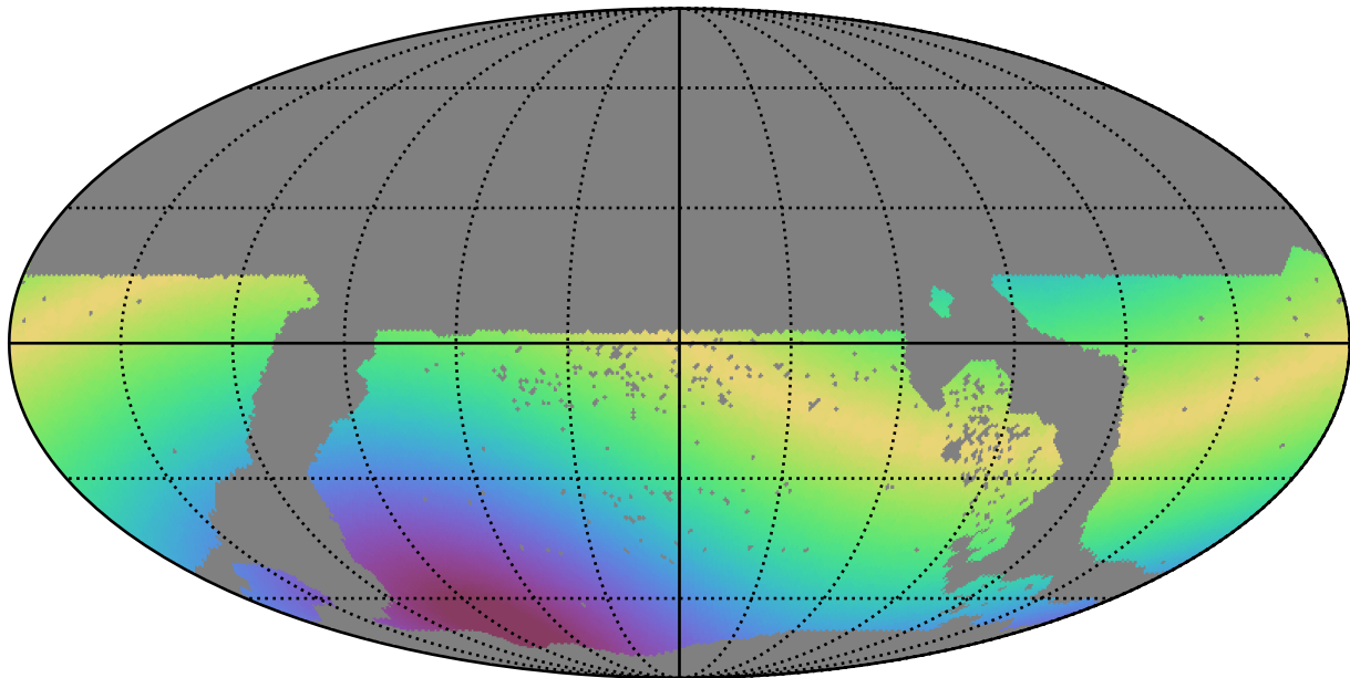
too_elab_r16_d2_gz_v3.4_10yrs WFD i band: Max solarElong
