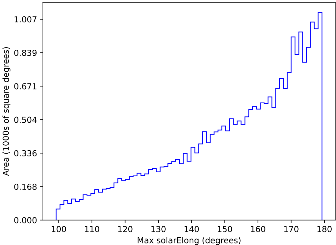
too_elab_r16_d2_gz_v3.4_10yrs All sky z band: Max solarElong
