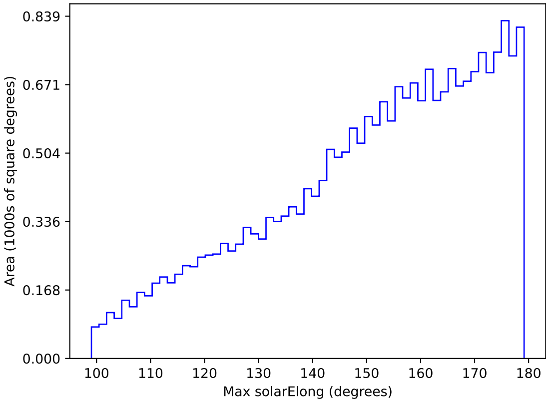
too_elab_r16_d2_gz_v3.4_10yrs All sky y band: Max solarElong
