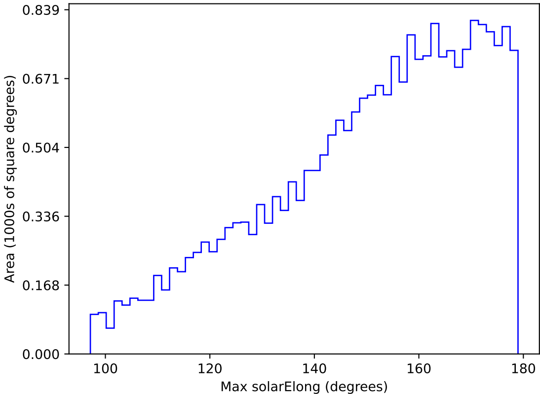
too_elab_r16_d2_gz_v3.4_10yrs All sky u band: Max solarElong
