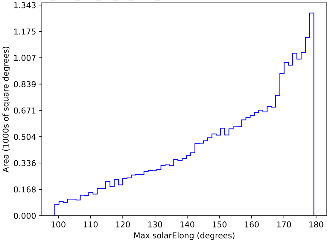
too_elab_r16_d2_gz_v3.4_10yrs All sky r band: Max solarElong
