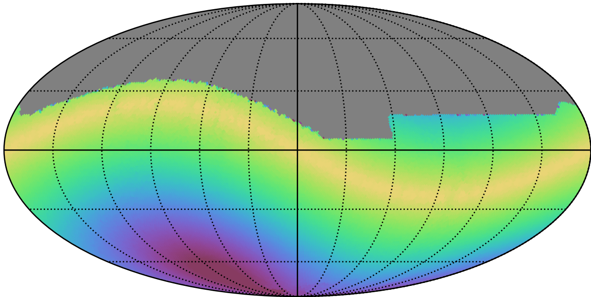
too_elab_r16_d2_gz_v3.4_10yrs All sky i band: Max solarElong
