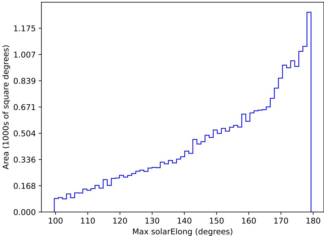
too_elab_r16_d2_gz_v3.4_10yrs All sky i band: Max solarElong
