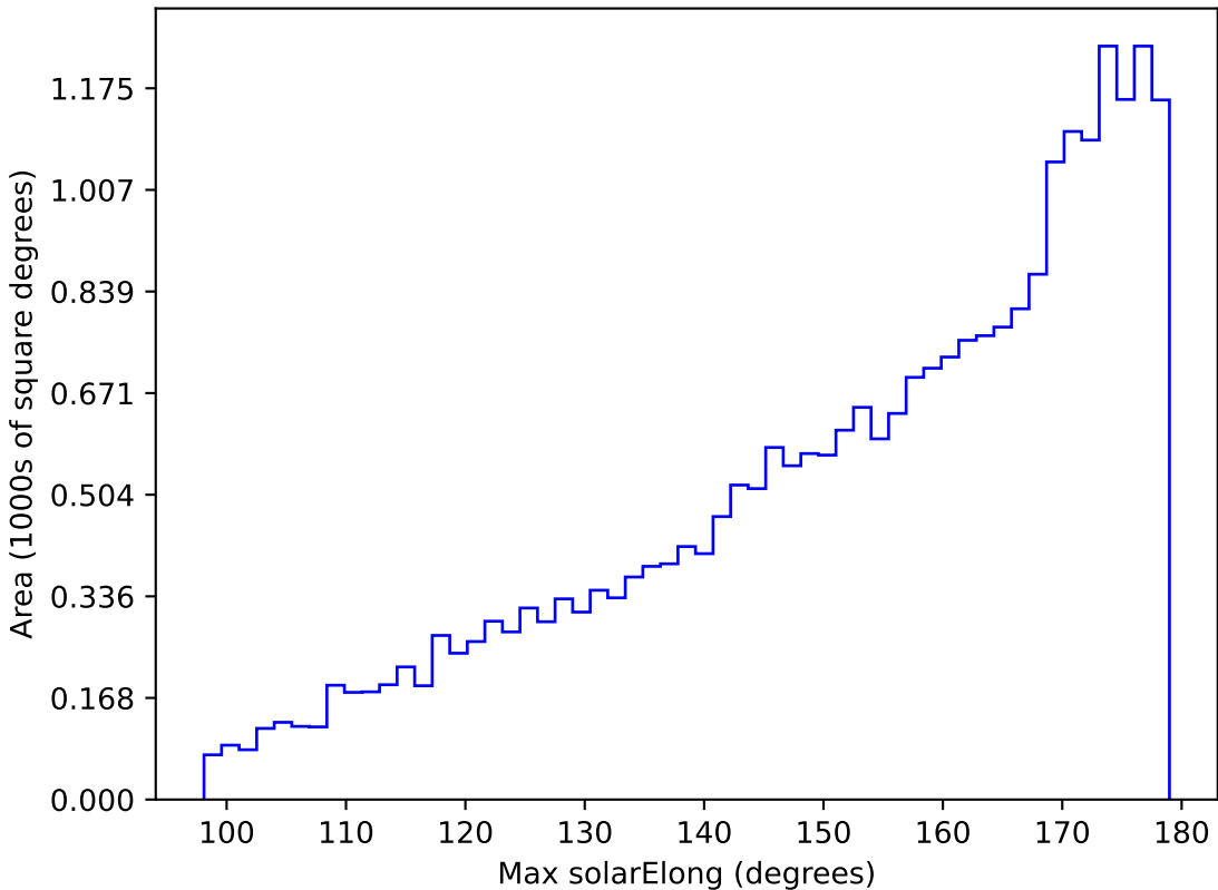
too_elab_r16_d2_gz_v3.4_10yrs All sky g band: Max solarElong
