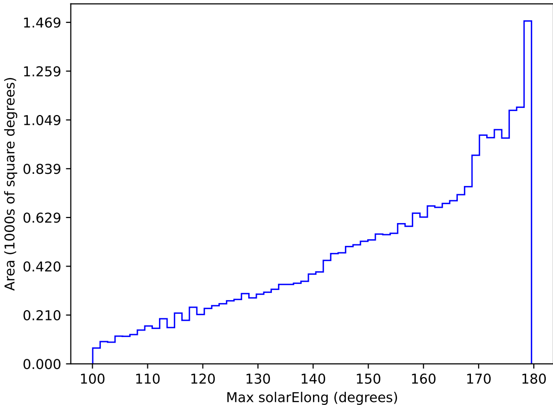
too_elab_r16_d2_gz_v3.4_10yrs All sky all bands: Max solarElong
