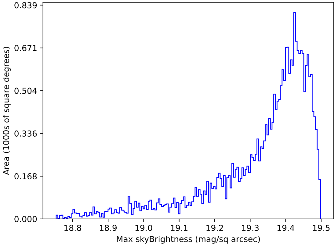
too_elab_r16_d2_gz_v3.4_10yrs Yr 1 z band: Max skyBrightness
