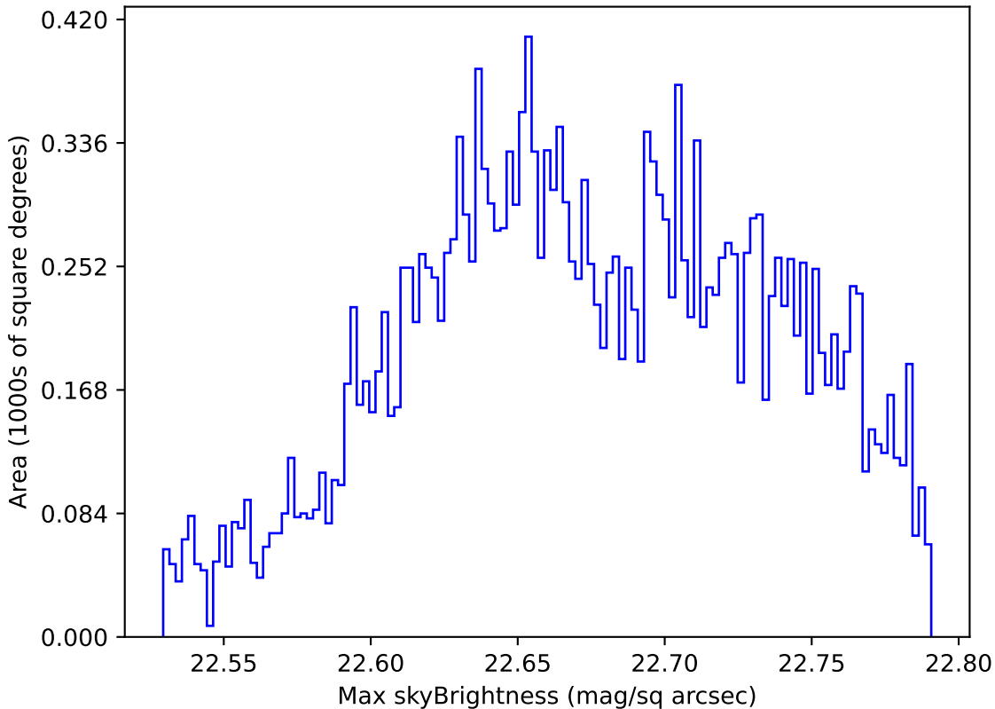
too_elab_r16_d2_gz_v3.4_10yrs Yr 1 u band: Max skyBrightness
