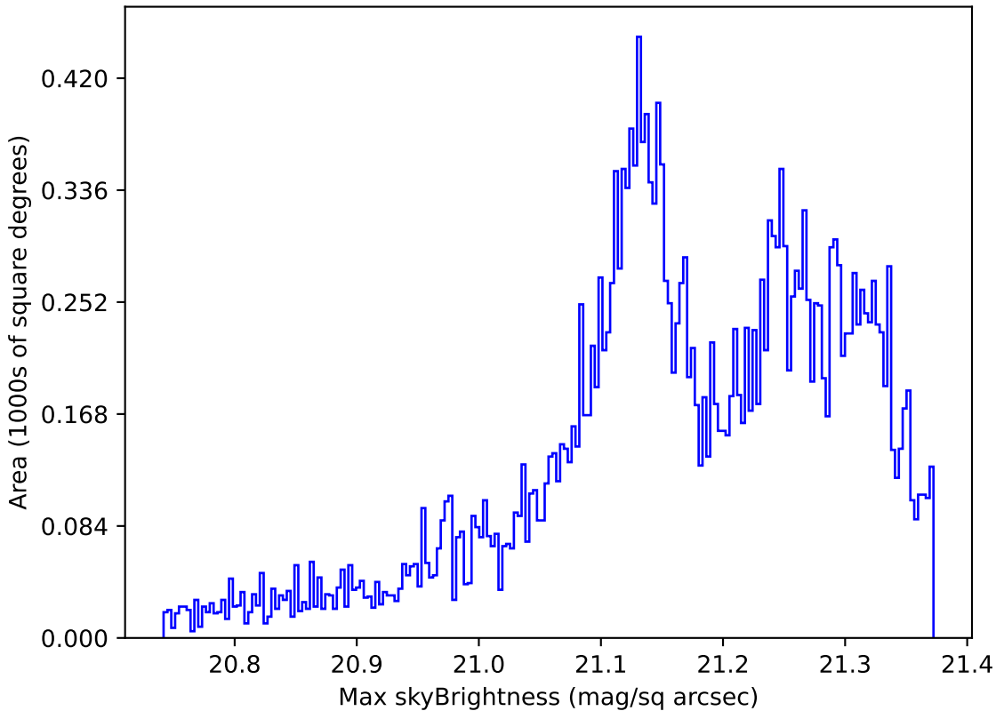
too_elab_r16_d2_gz_v3.4_10yrs Yr 1 r band: Max skyBrightness
