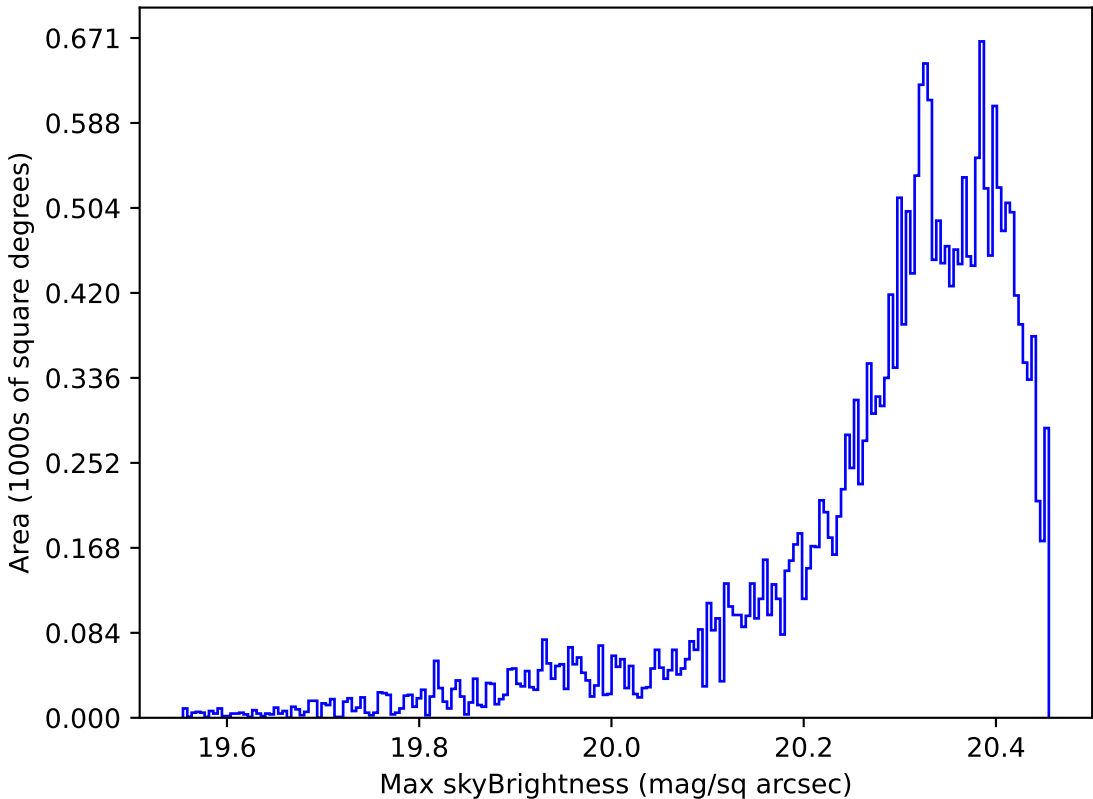
too_elab_r16_d2_gz_v3.4_10yrs Yr 1 i band: Max skyBrightness
