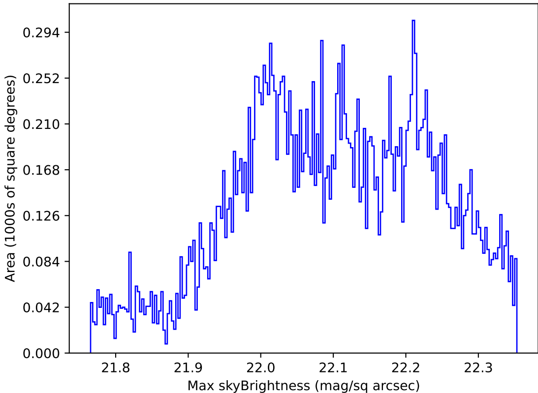
too_elab_r16_d2_gz_v3.4_10yrs Yr 1 g band: Max skyBrightness
