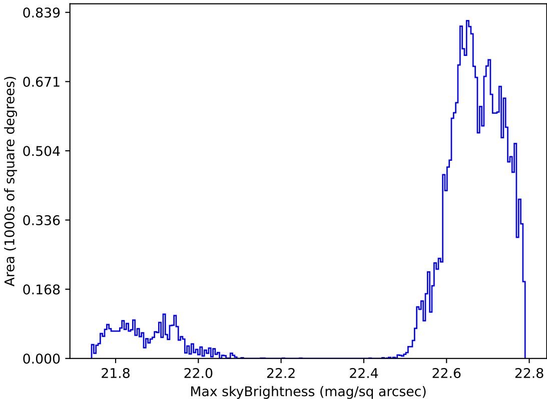
too_elab_r16_d2_gz_v3.4_10yrs Yr 1 all bands: Max skyBrightness
