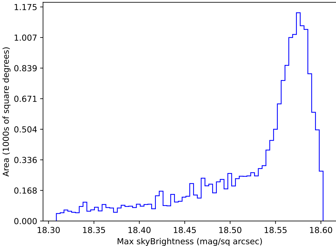
too_elab_r16_d2_gz_v3.4_10yrs WFD y band: Max skyBrightness
