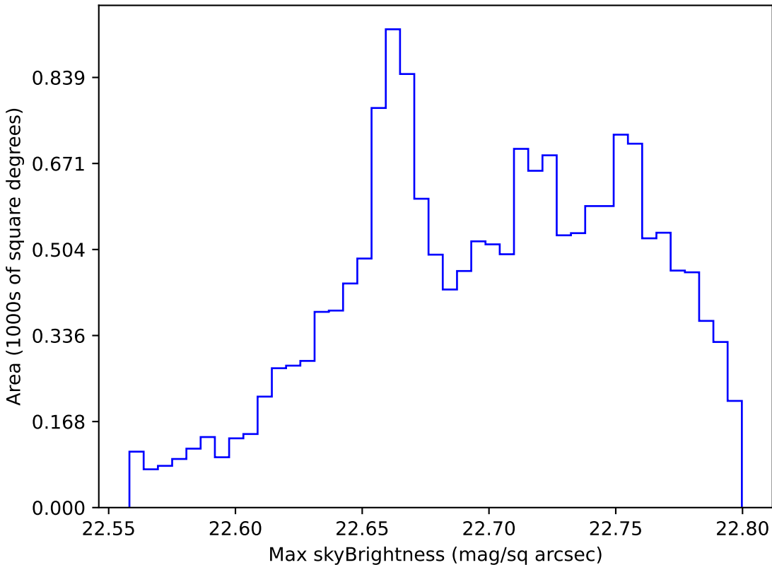
too_elab_r16_d2_gz_v3.4_10yrs WFD u band: Max skyBrightness
