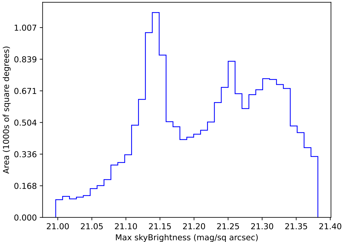
too_elab_r16_d2_gz_v3.4_10yrs WFD r band: Max skyBrightness
