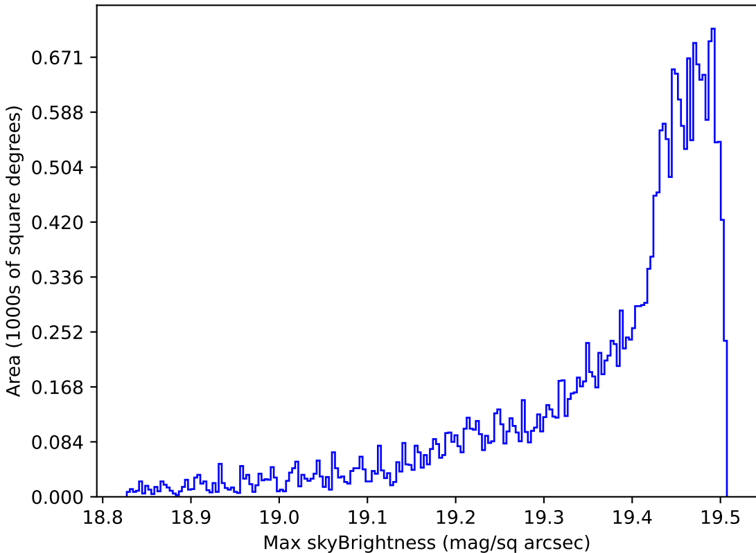
too_elab_r16_d2_gz_v3.4_10yrs All sky z band: Max skyBrightness
