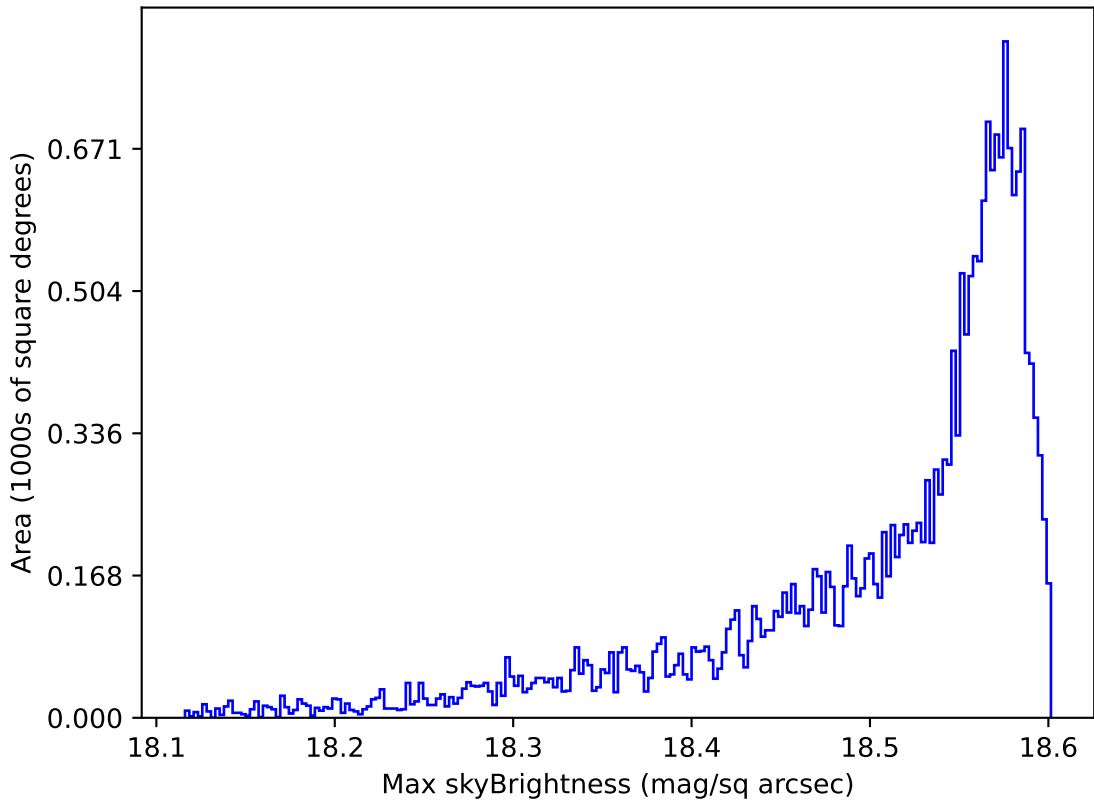
too_elab_r16_d2_gz_v3.4_10yrs All sky y band: Max skyBrightness
