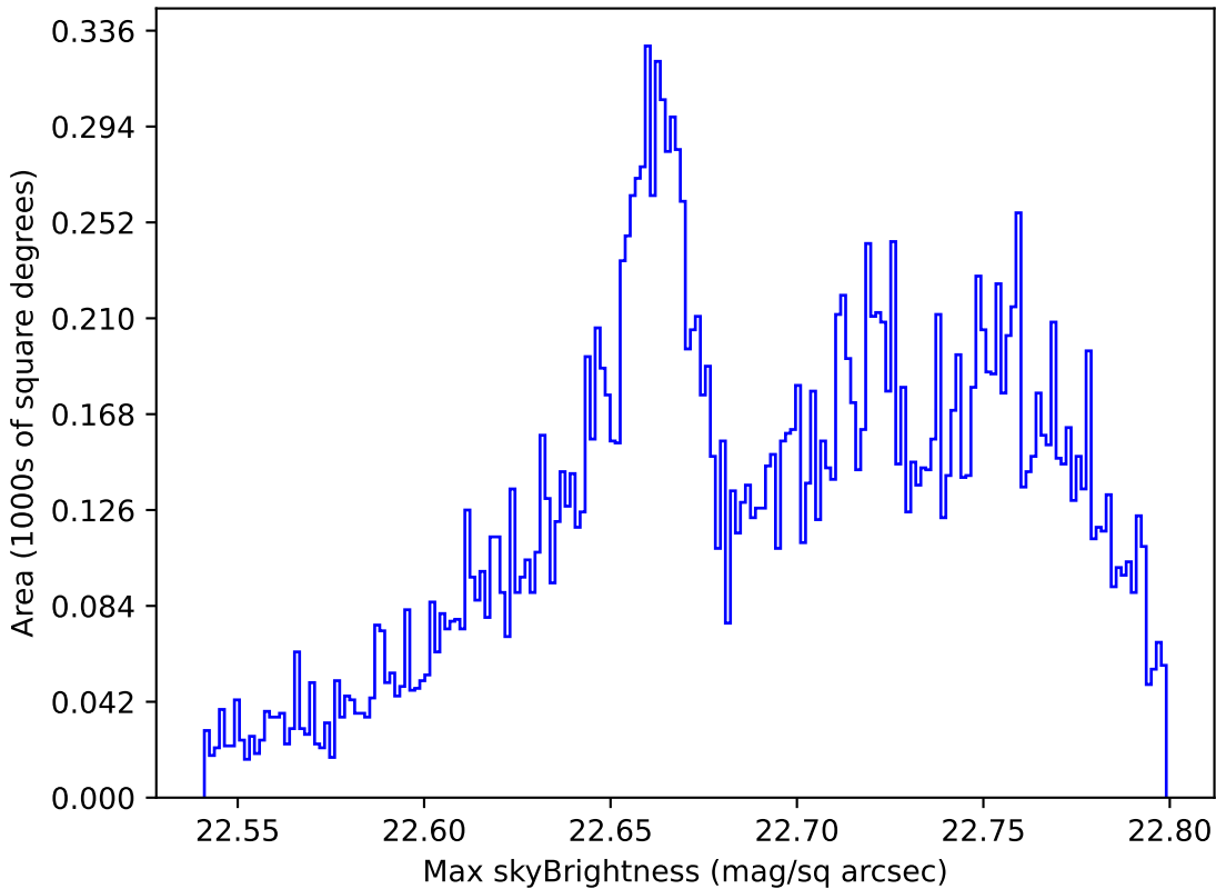
too_elab_r16_d2_gz_v3.4_10yrs All sky u band: Max skyBrightness
