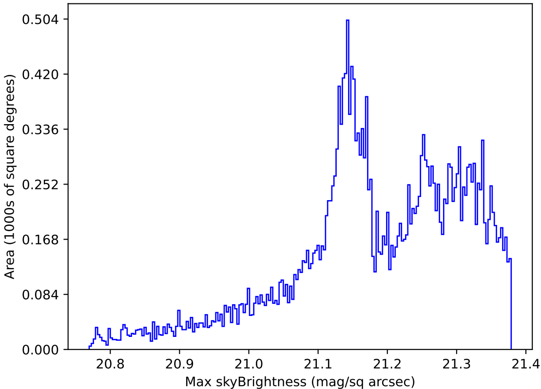
too_elab_r16_d2_gz_v3.4_10yrs All sky r band: Max skyBrightness
