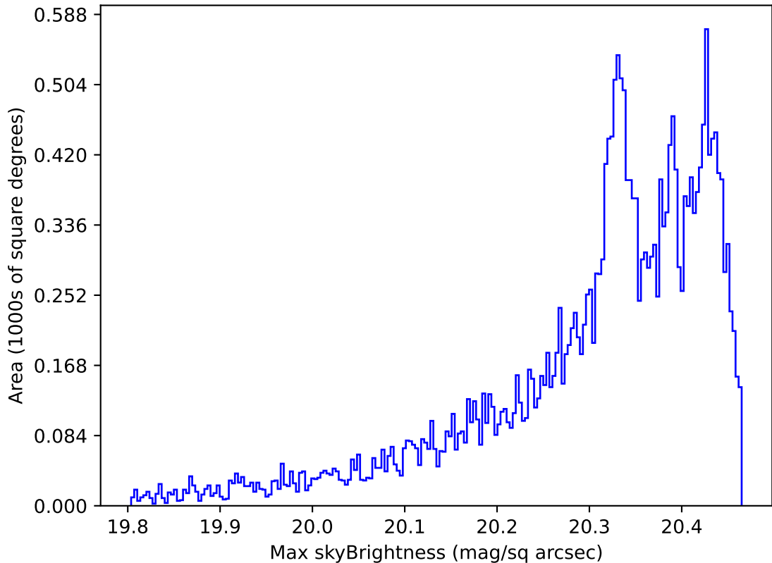
too_elab_r16_d2_gz_v3.4_10yrs All sky i band: Max skyBrightness
