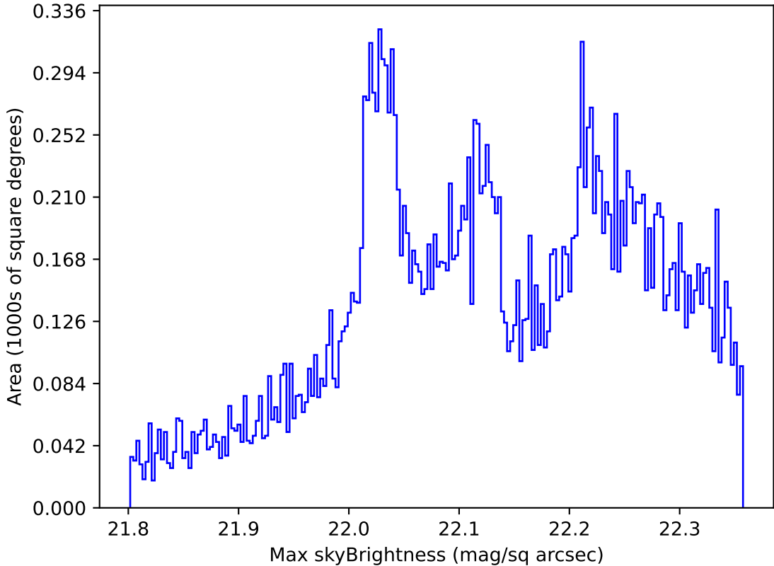
too_elab_r16_d2_gz_v3.4_10yrs All sky g band: Max skyBrightness
