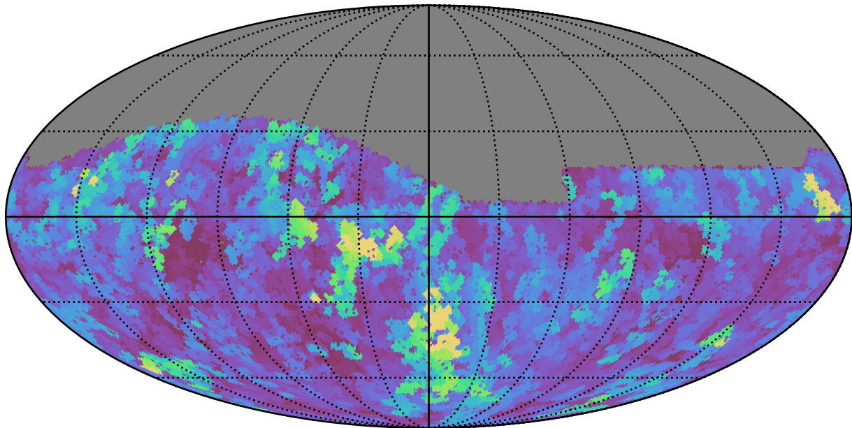
too_elab_r16_d2_gz_v3.4_10yrs Yr 1 z band: Max seeingGeom
