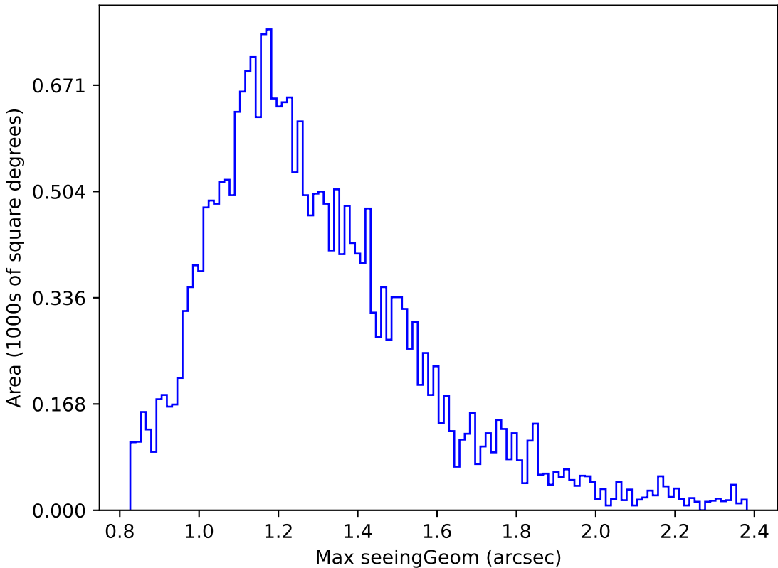
too_elab_r16_d2_gz_v3.4_10yrs Yr 1 z band: Max seeingGeom
