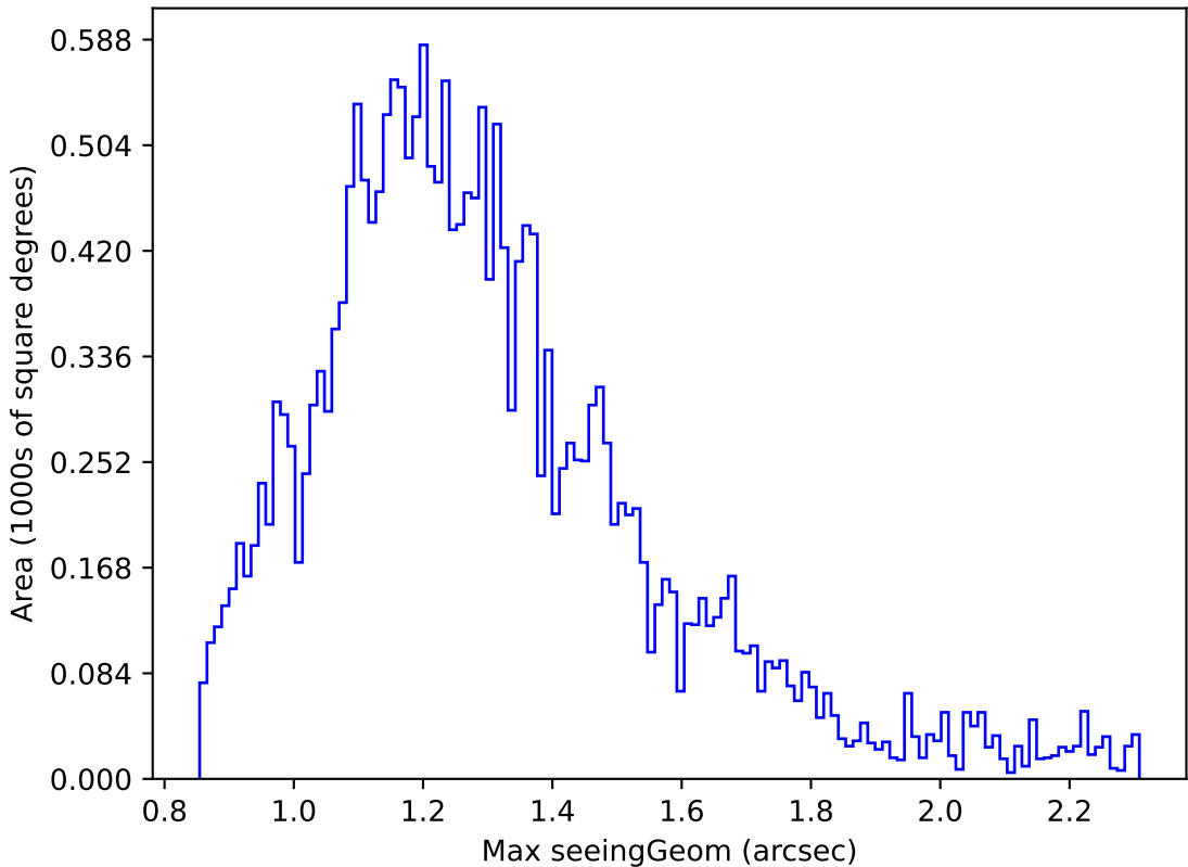
too_elab_r16_d2_gz_v3.4_10yrs Yr 1 y band: Max seeingGeom
