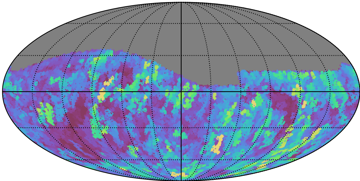
too_elab_r16_d2_gz_v3.4_10yrs Yr 1 r band: Max seeingGeom
