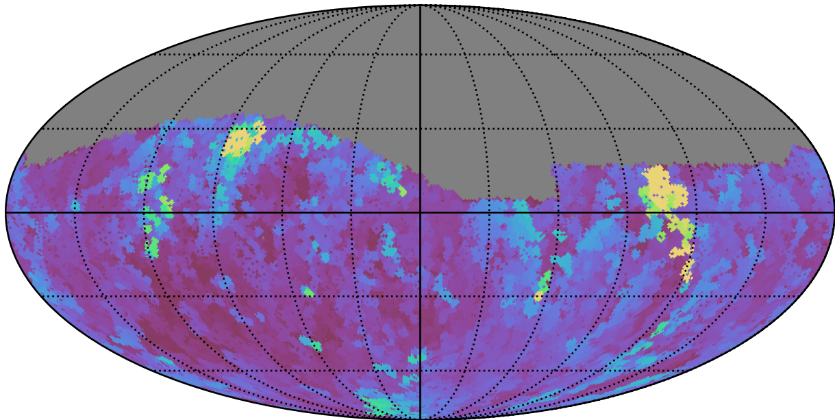
too_elab_r16_d2_gz_v3.4_10yrs Yr 1 g band: Max seeingGeom
