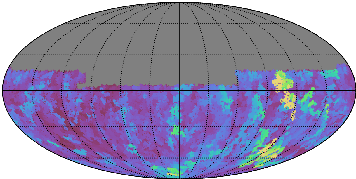
too_elab_r16_d2_gz_v3.4_10yrs Yr 1 u band: Max seeingEff
