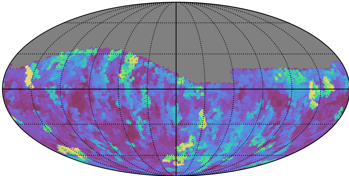
too_elab_r16_d2_gz_v3.4_10yrs Yr 1 i band: Max seeingEff
