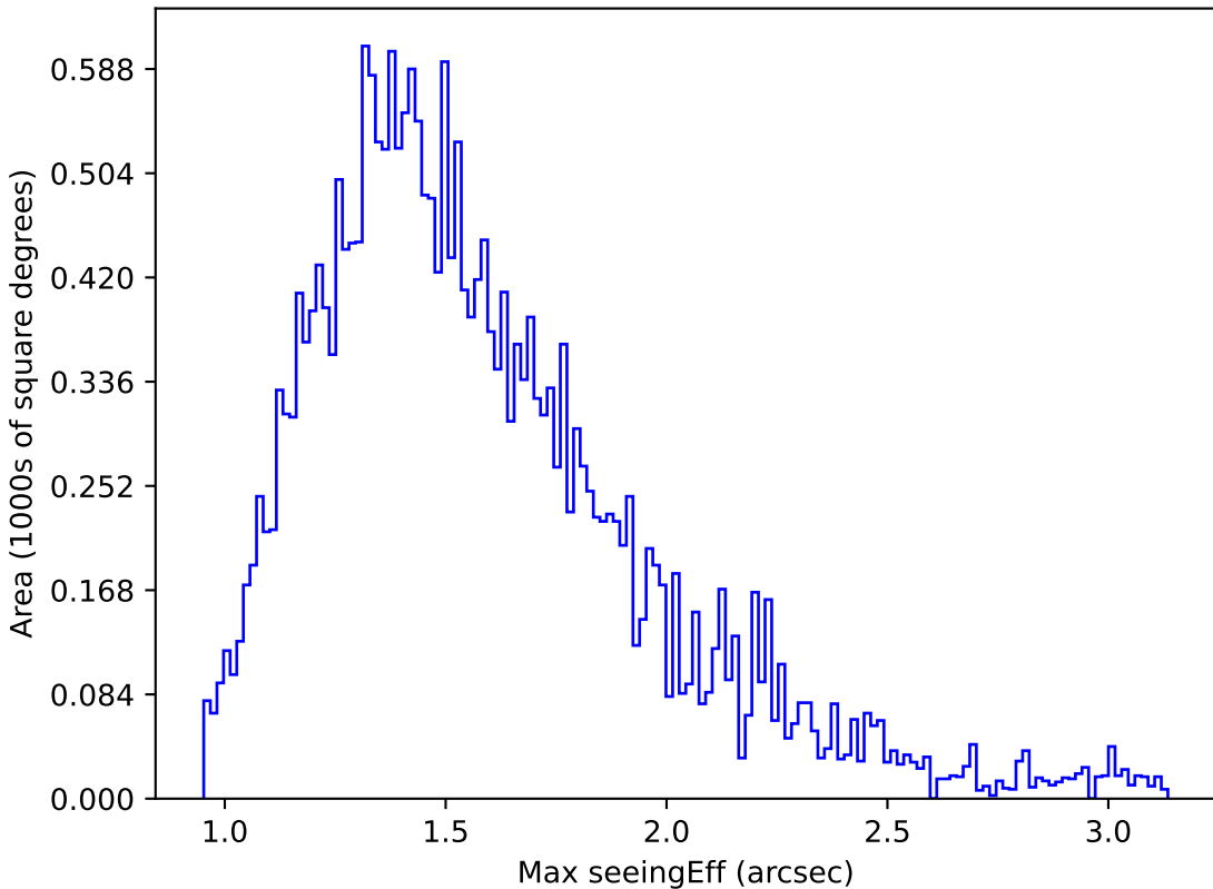
too_elab_r16_d2_gz_v3.4_10yrs Yr 1 i band: Max seeingEff
