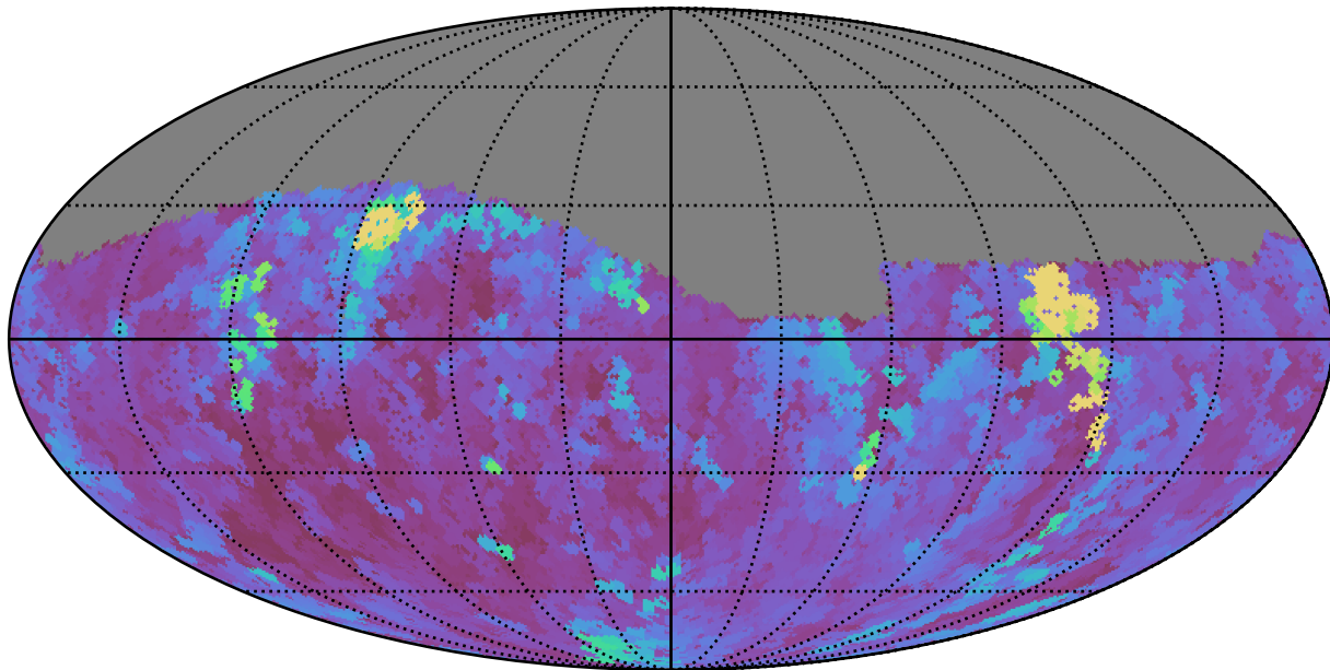
too_elab_r16_d2_gz_v3.4_10yrs Yr 1 g band: Max seeingEff
