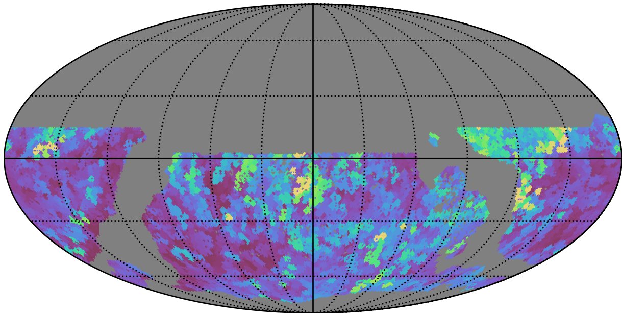
too_elab_r16_d2_gz_v3.4_10yrs WFD r band: Max seeingEff
