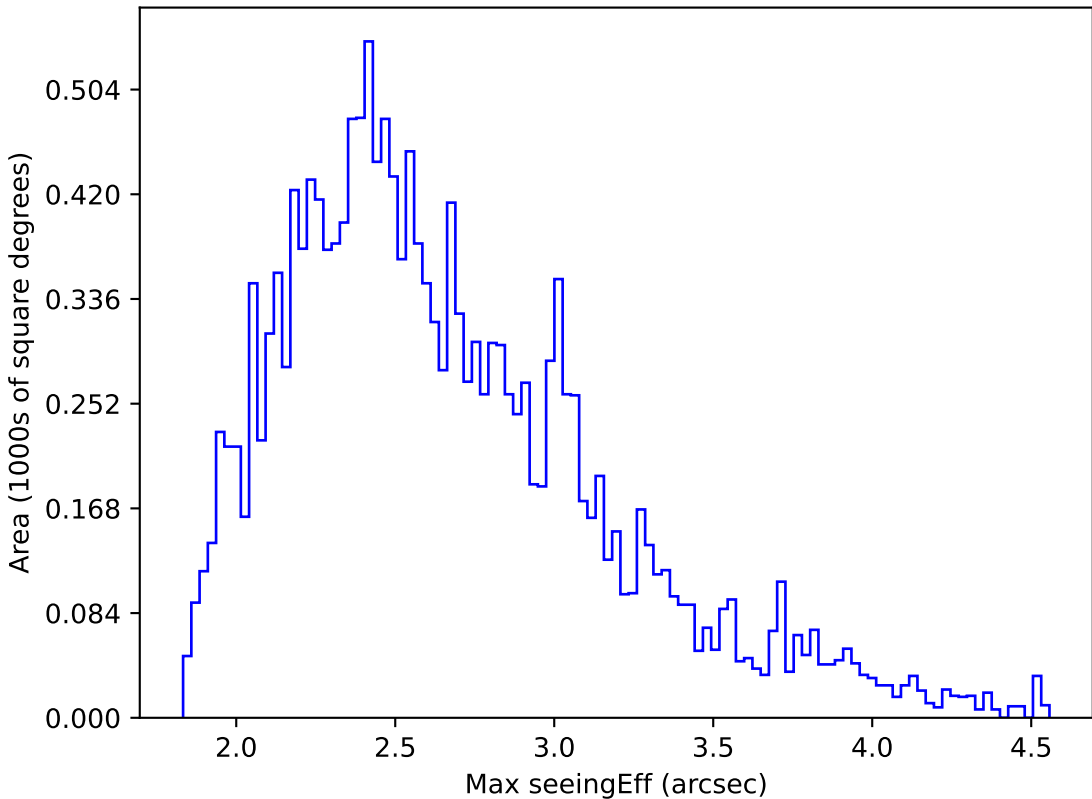
too_elab_r16_d2_gz_v3.4_10yrs WFD r band: Max seeingEff
