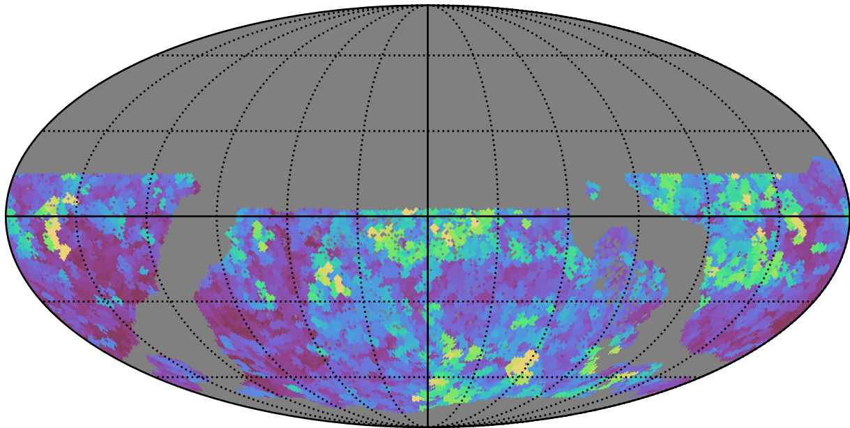
too_elab_r16_d2_gz_v3.4_10yrs WFD all bands: Max seeingEff
