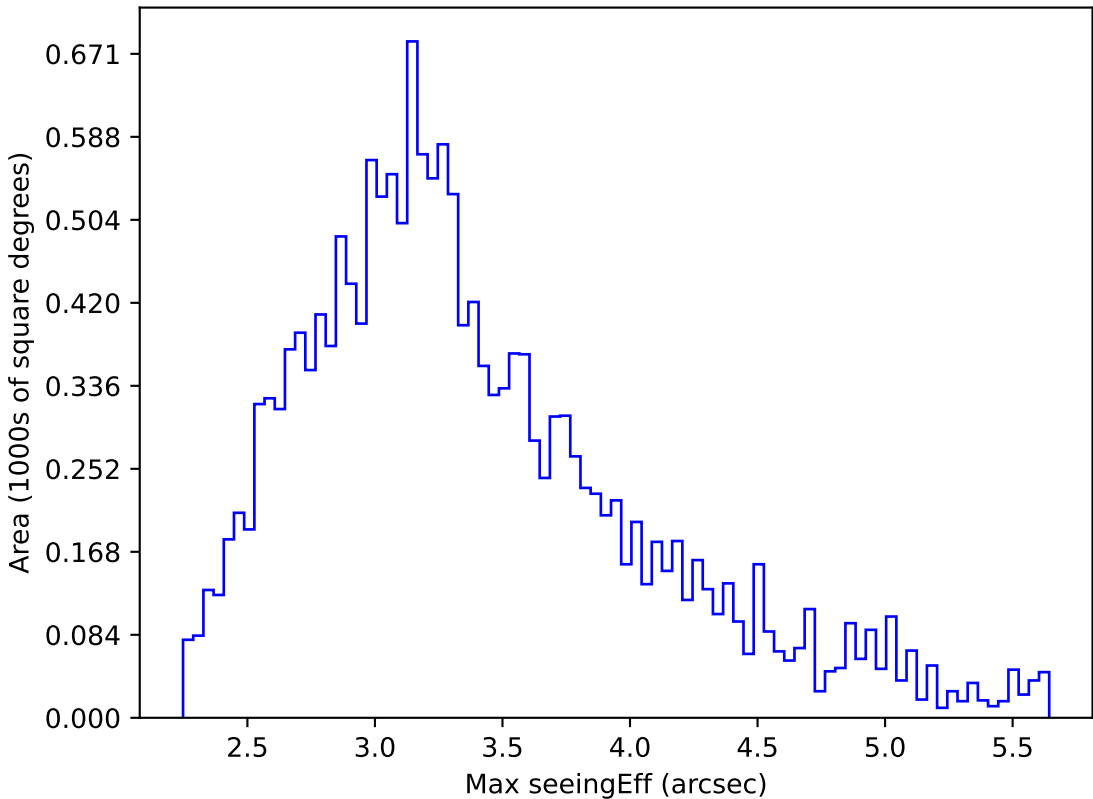
too_elab_r16_d2_gz_v3.4_10yrs WFD all bands: Max seeingEff
