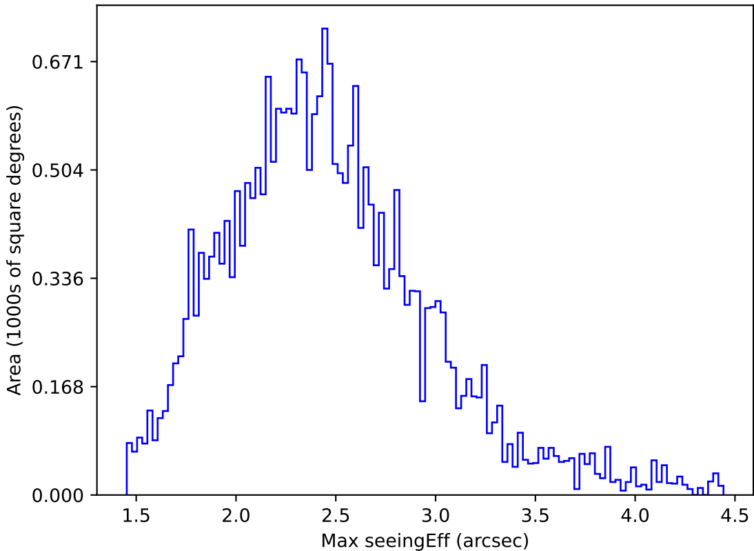
too_elab_r16_d2_gz_v3.4_10yrs All sky z band: Max seeingEff
