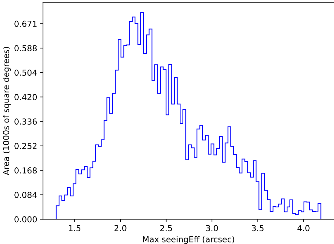
too_elab_r16_d2_gz_v3.4_10yrs All sky u band: Max seeingEff
