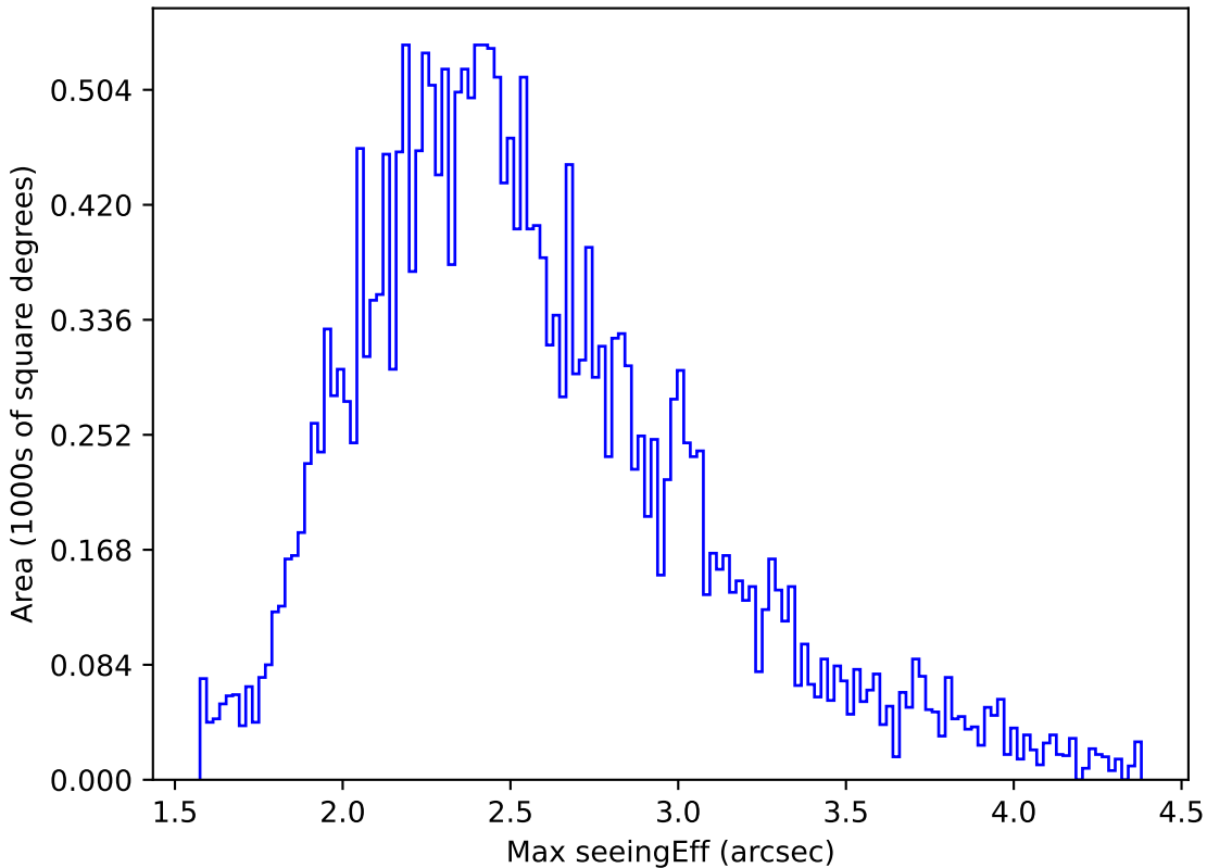
too_elab_r16_d2_gz_v3.4_10yrs All sky r band: Max seeingEff
