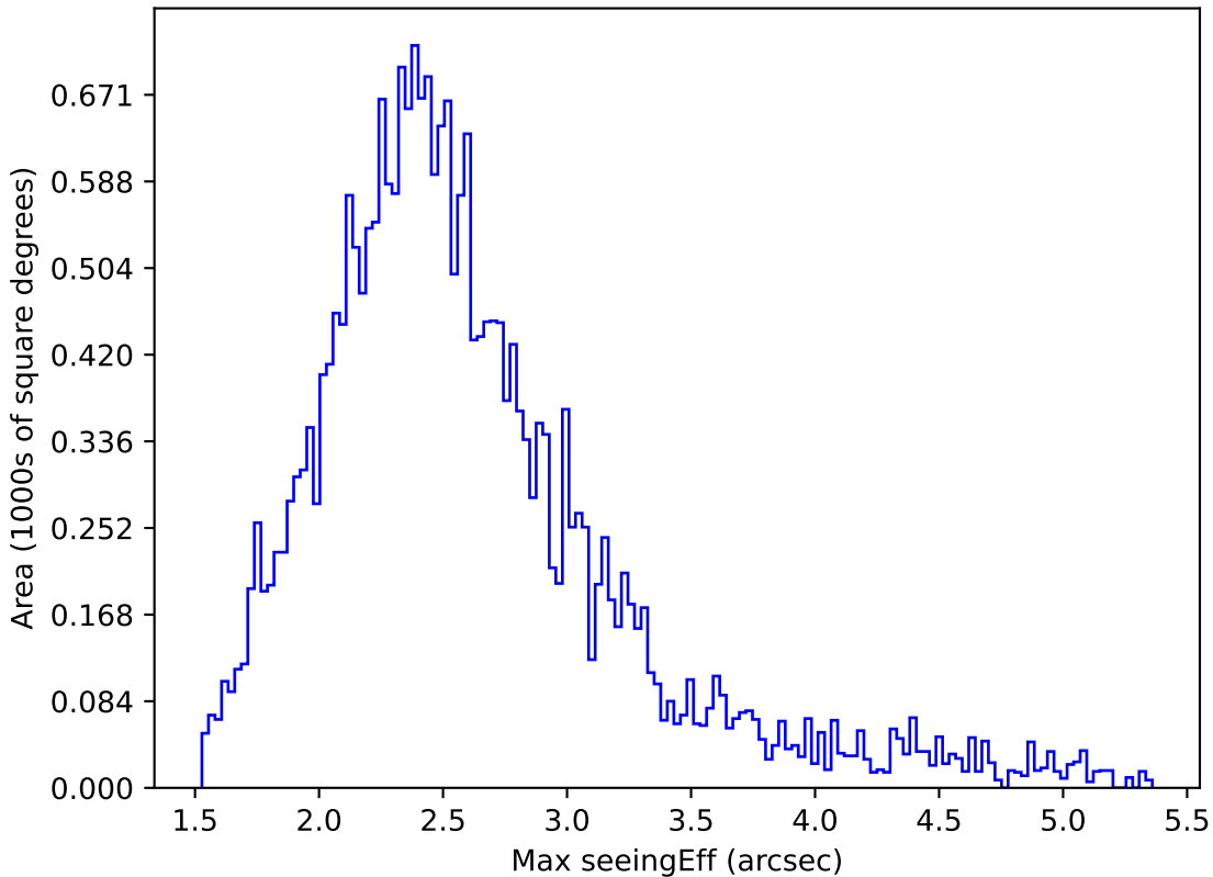
too_elab_r16_d2_gz_v3.4_10yrs All sky i band: Max seeingEff
