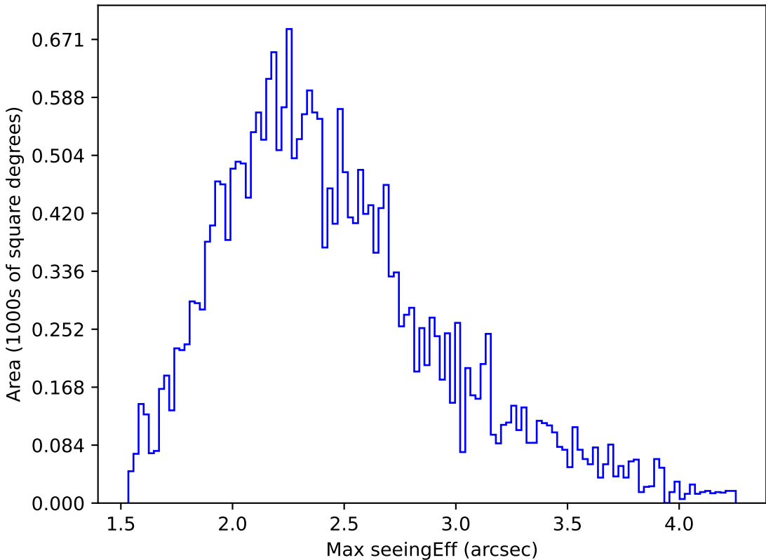
too_elab_r16_d2_gz_v3.4_10yrs All sky g band: Max seeingEff
