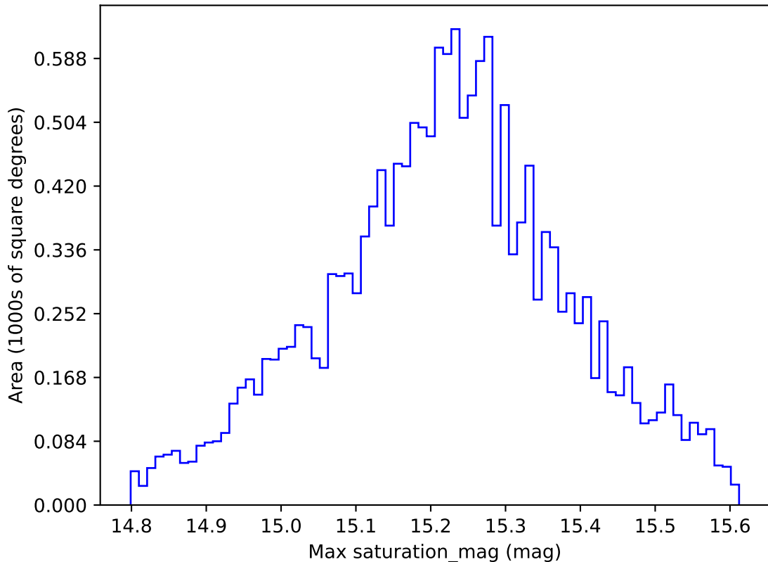
too_elab_r16_d2_gz_v3.4_10yrs WFD z band: Max saturation_mag
