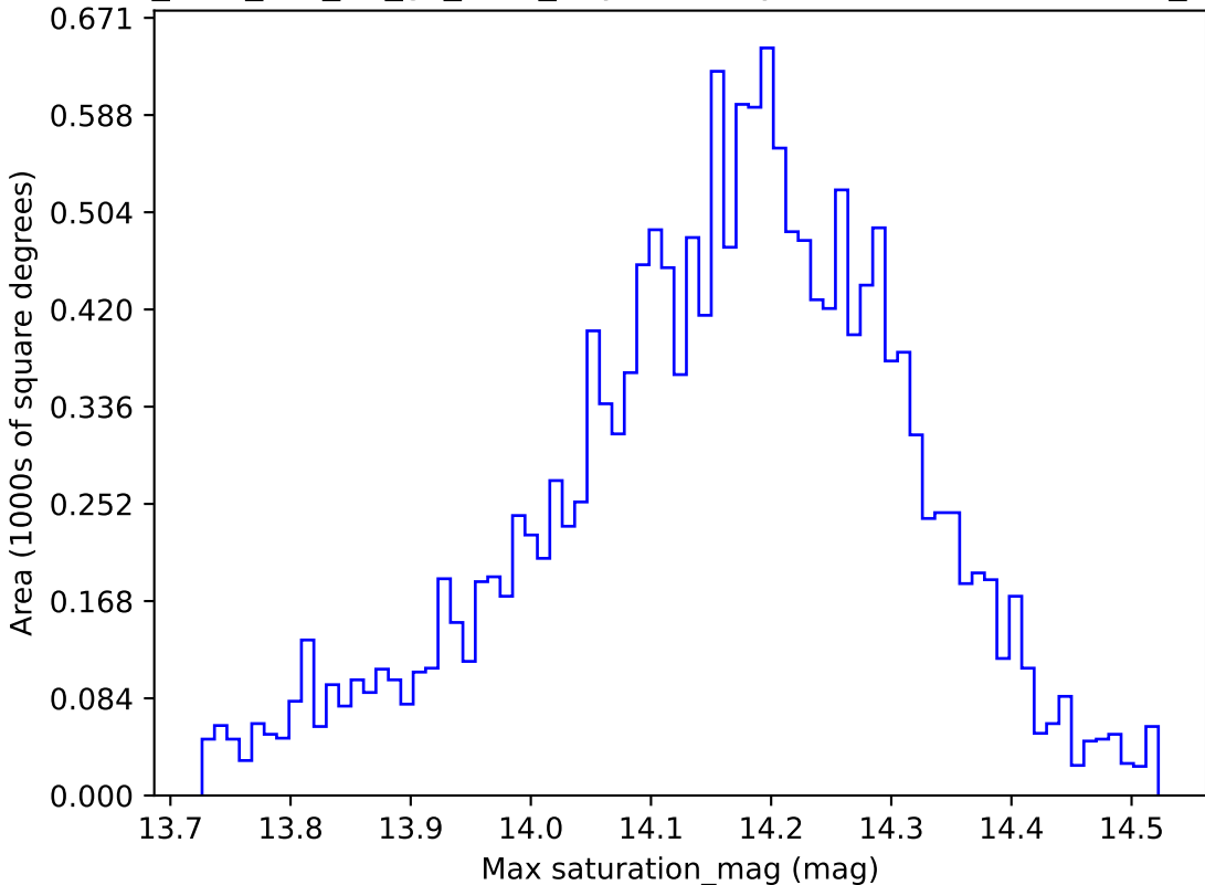
too_elab_r16_d2_gz_v3.4_10yrs WFD y band: Max saturation_mag
